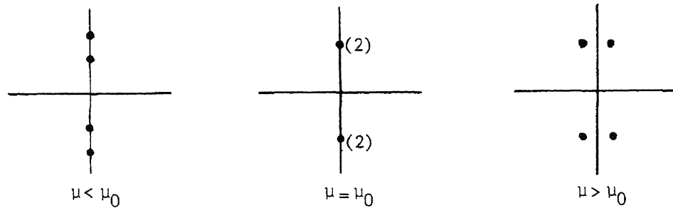
Figure 2 The eigenvalues of the linearized system in the complex plane.
